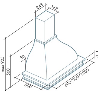
parete/wall
